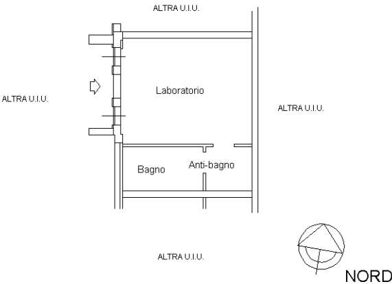
Pianta Piano Seminterrato (S1) h=mt.2.70
